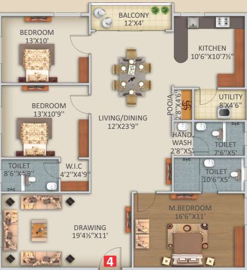
3BHK West | 1885sft
